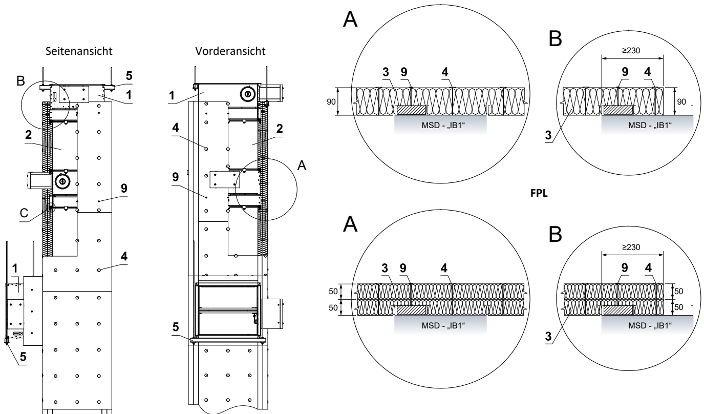
Flame Shield
