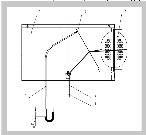
Fig. 7 plenum box with the regulation dampers control by means of ropes and with pressure probe - supply
