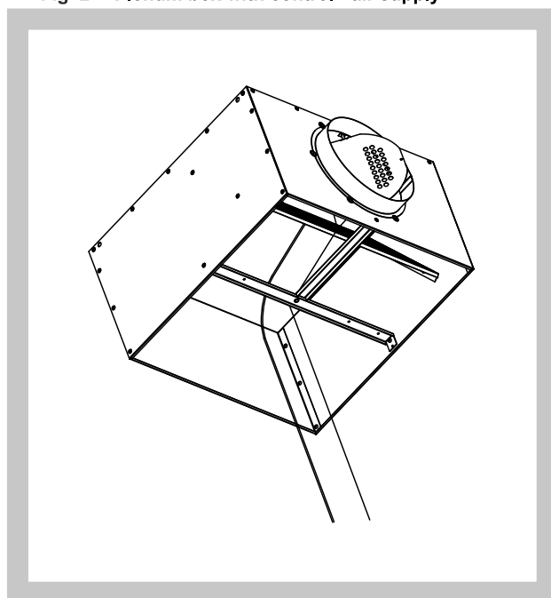
Fig. 2 Plenum box with control - air supply
