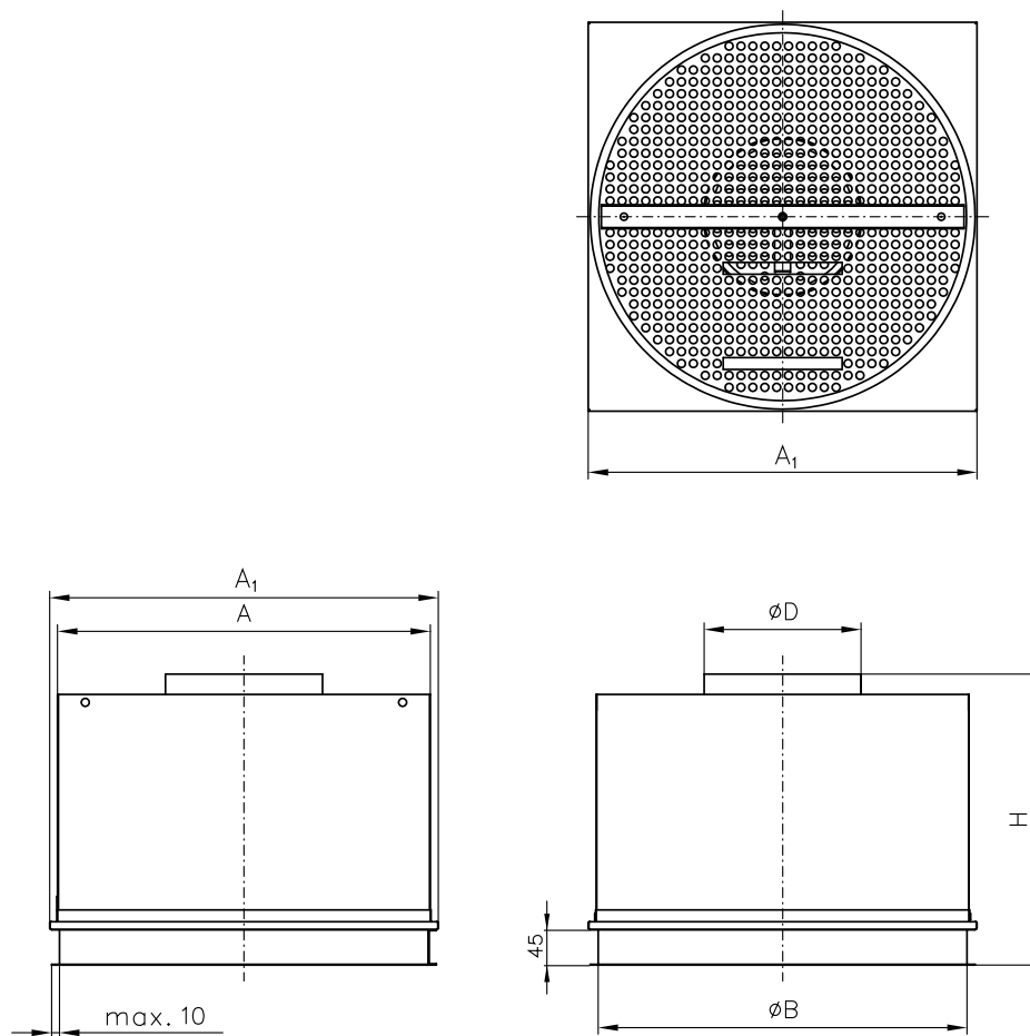
Fig. 6 Vertical connection, circular front panel
