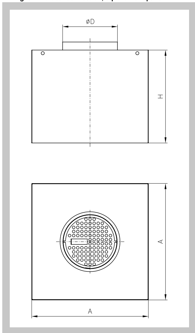
Fig. 5 Vertical connection, square front panel
